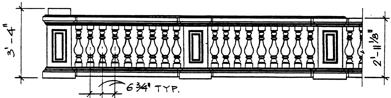
ELEVATION OF BALUSTRADE
