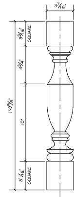
2 ELEVATION OF BALUSTER 3 SCALE: NTS
