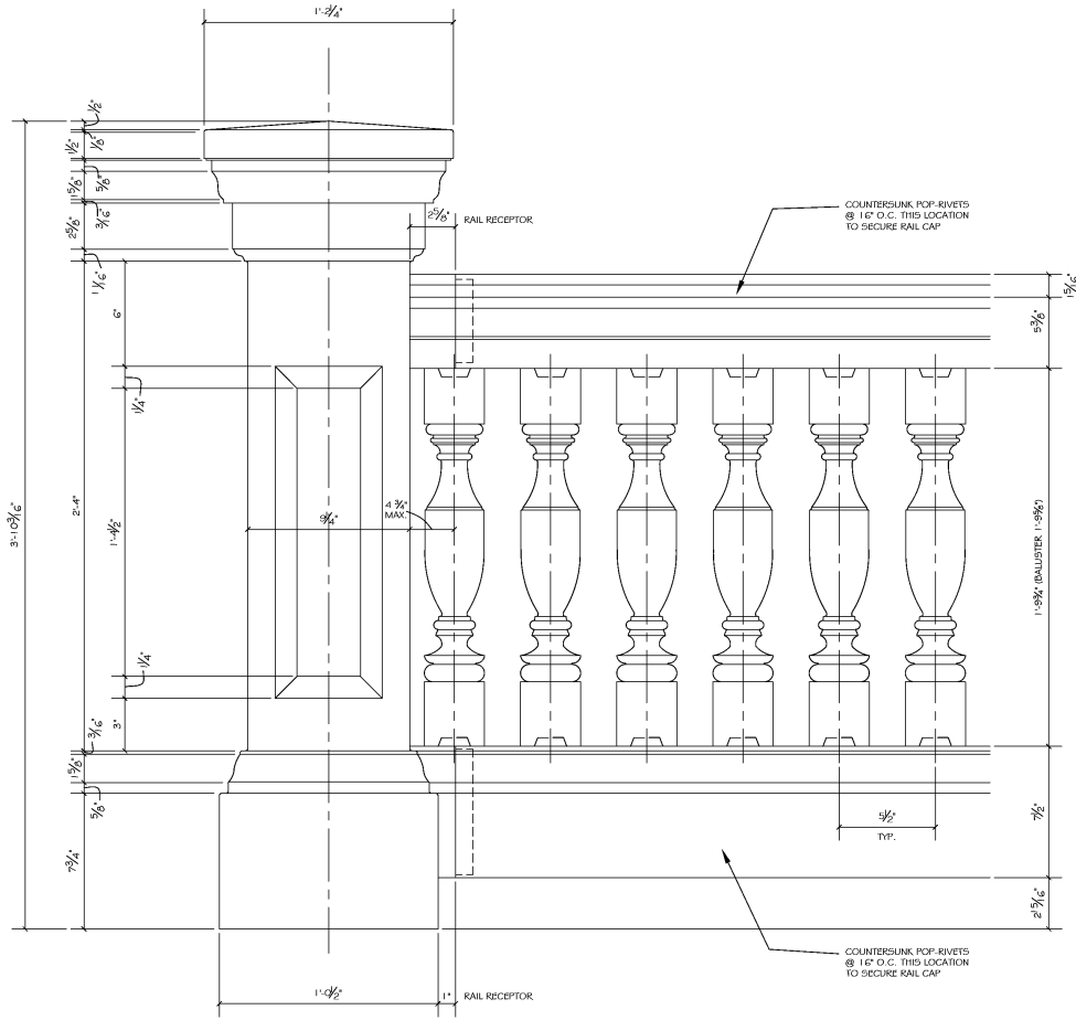
1 ELEVATION OF BALUSTRADE SYSTEM 3 SCALE: NTS
