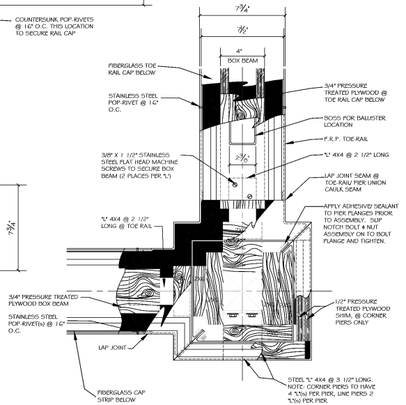
4 PLAN SECTION OF PIER 3 SCALE: NTS
