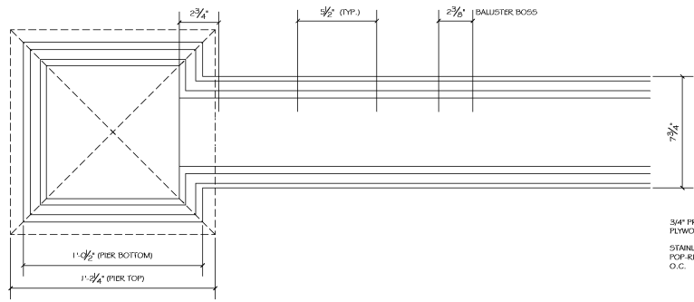
3 PLAN OF PIER/ RAILING 3 SCALE: NTS
