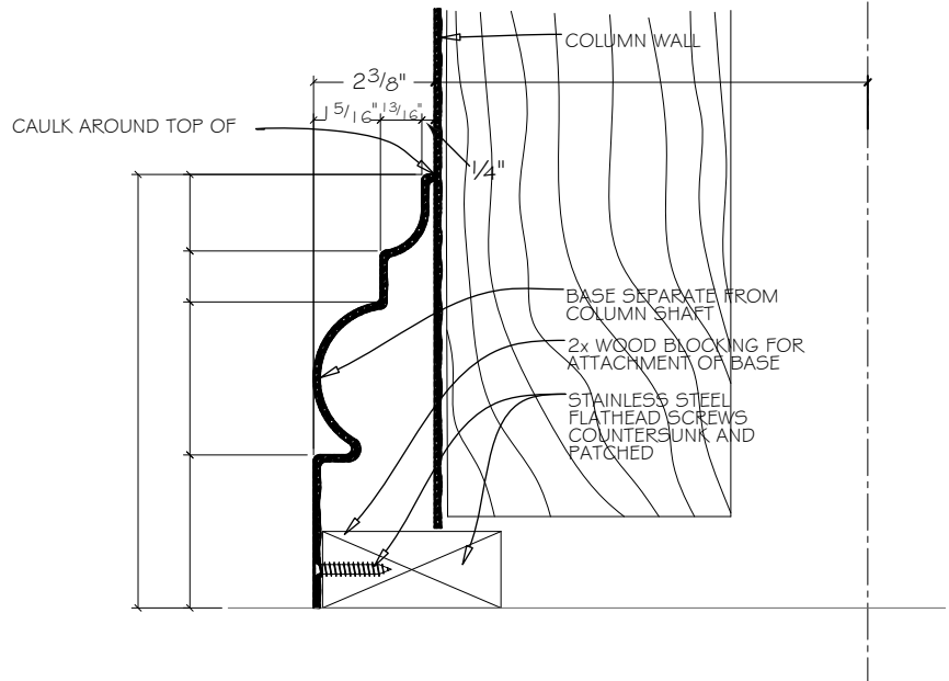
EC-120J.1 17" DIA. TUSCAN W/ENTASIS COLUMN COVER
