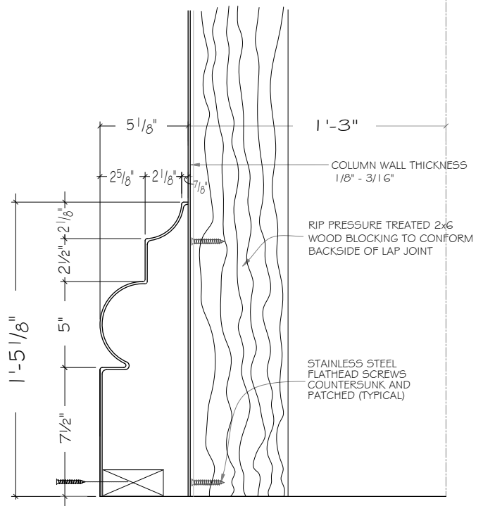
SECTION @ BASE
