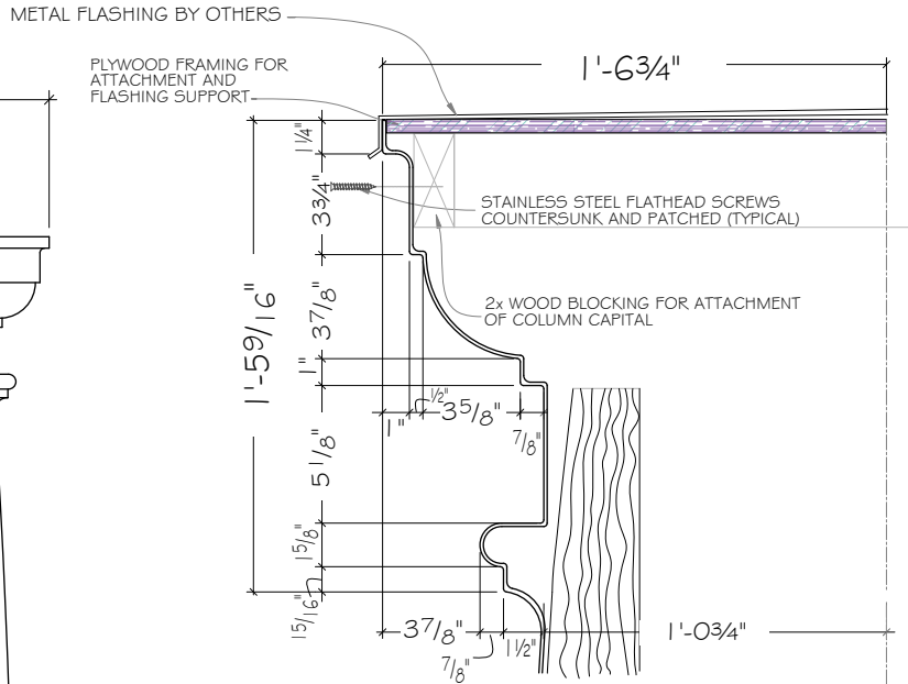
SECTION @ COLUMN CAPITAL
