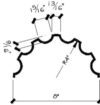
PLAN OF COLUMN SHAFT
