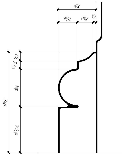
ELEVATION @ COLUMN BASE
