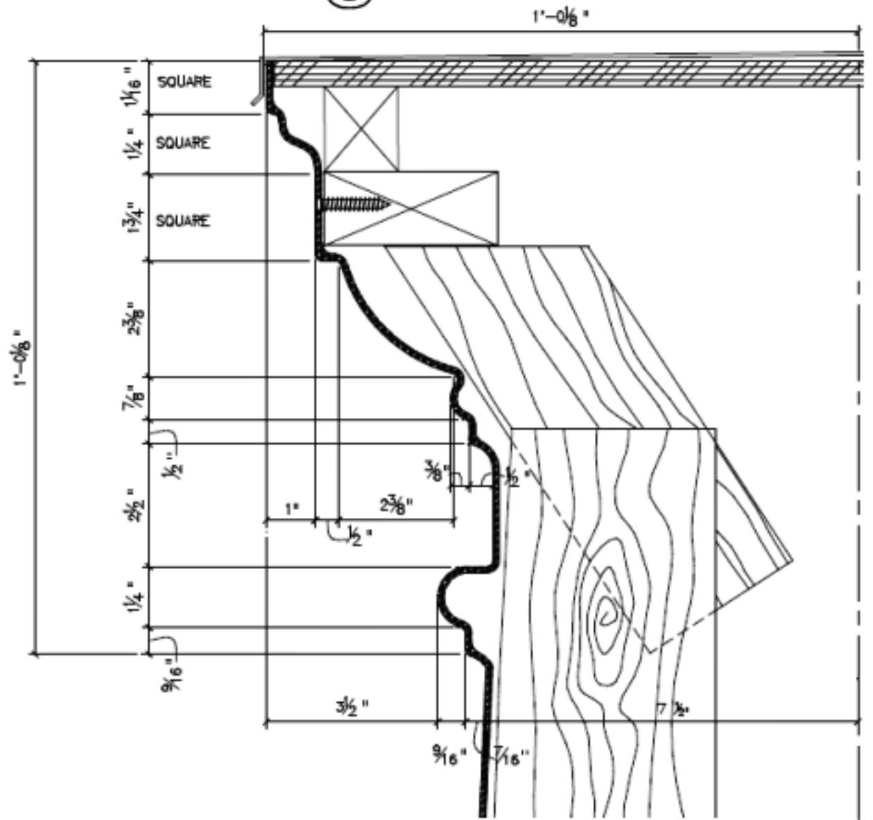
SECTION @ COLUMN CAPITAL
