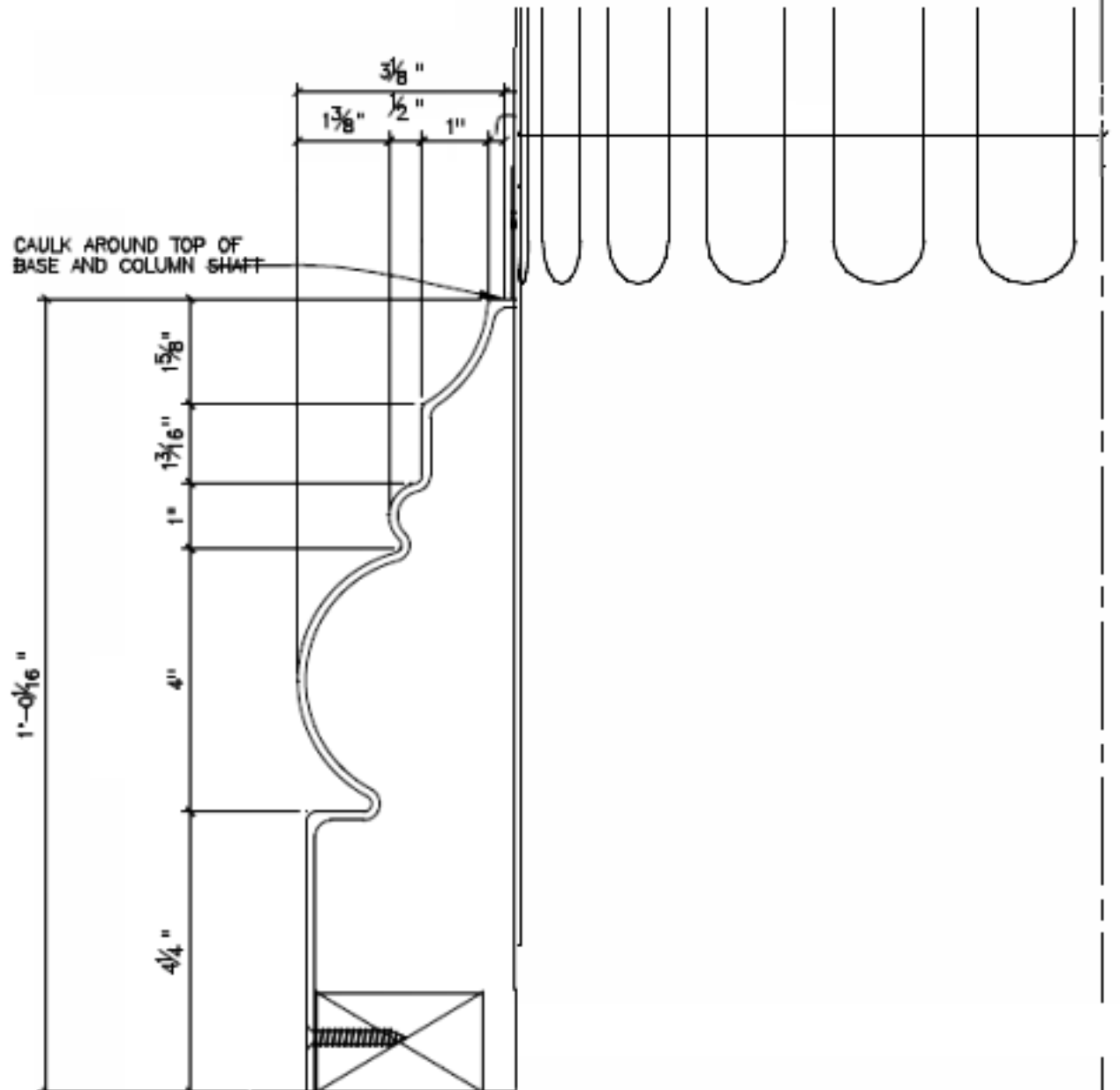
SECTION @ COLUMN BASE
