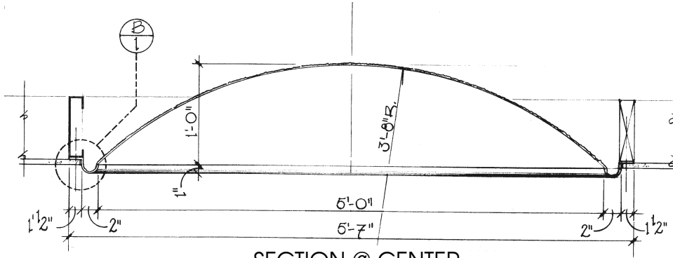
SECTION @ CENTER
