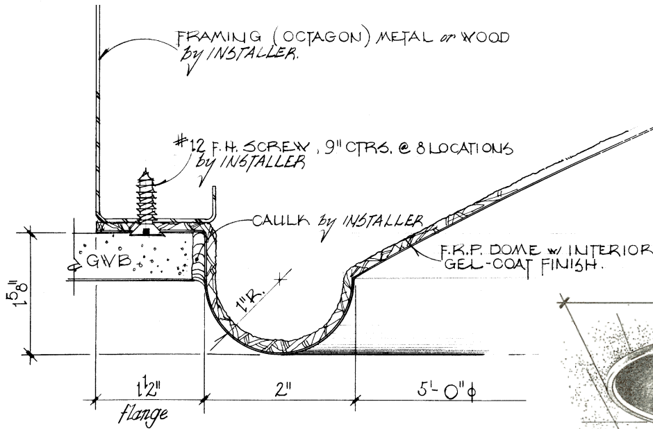
B 1 DETAIL: DOME MOUNTING NOTE: SKETCH ONLY NO SCALE
