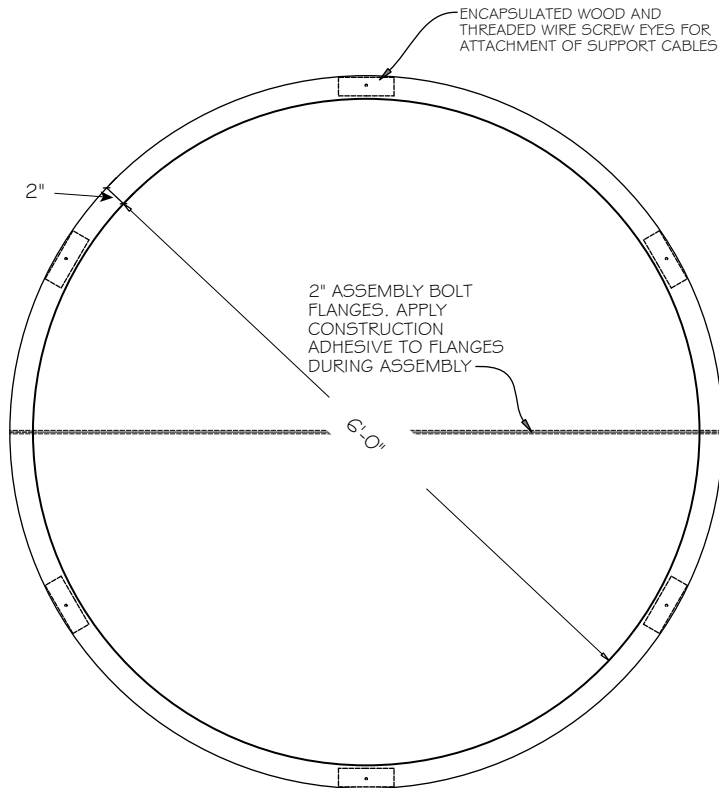
REFLECTED PLAN OF DOME
