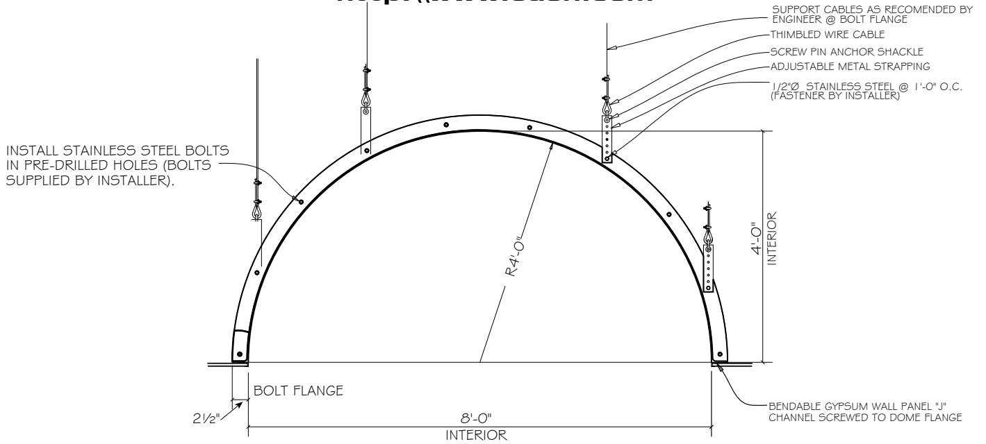
SECTION OF 8' DIA. INTERIOR DOME
