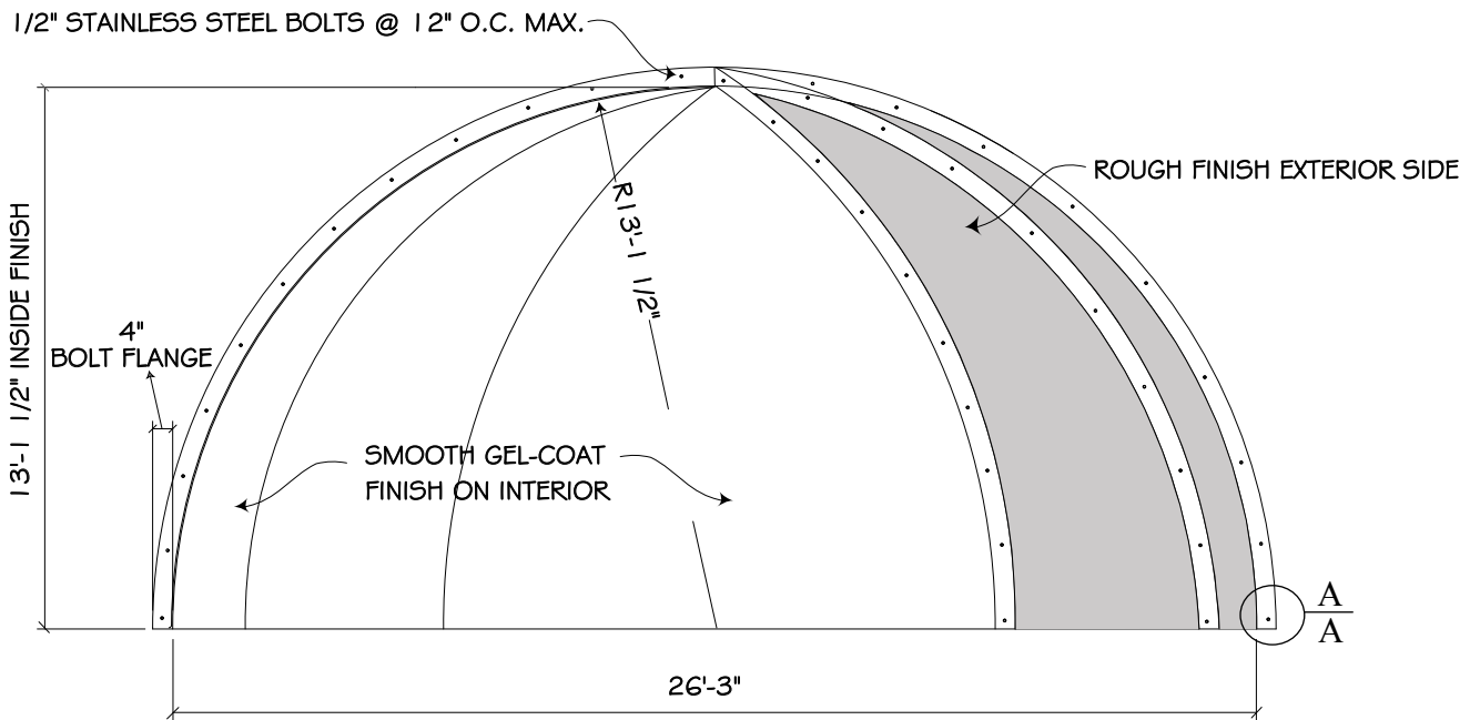
SECTION / ELEVATION
