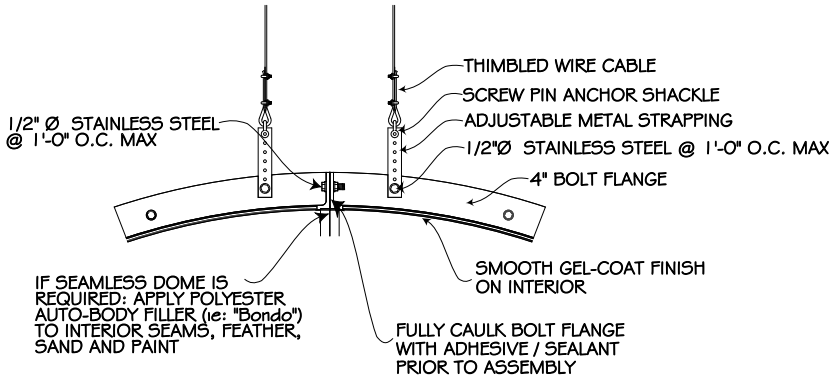
HANGING FLANGE DETAIL
