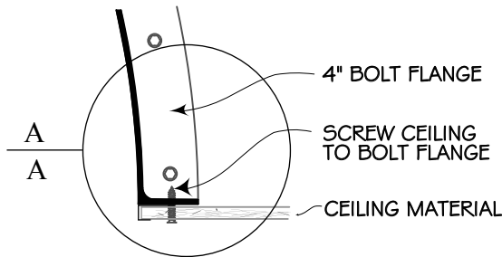
CEILING ATTACHMENT
