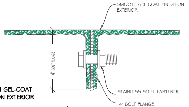
BOLT FLANGE DETAIL
