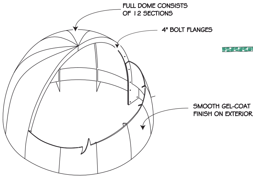
DOMES PLAN DETAIL
