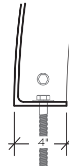
BASE BOLT FLANGE DETAIL
