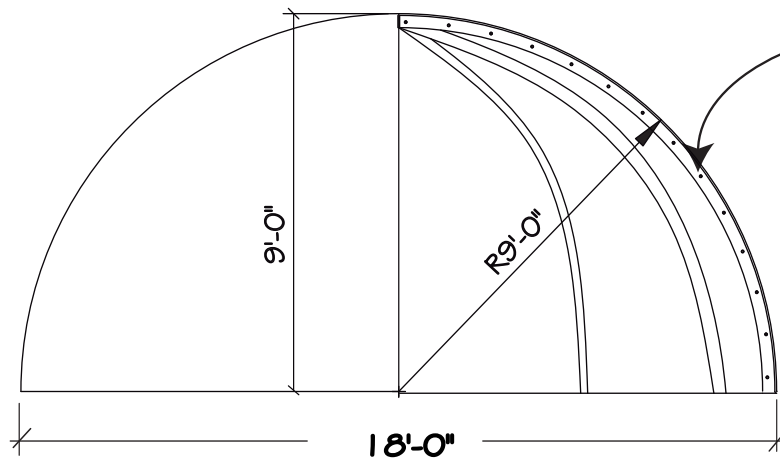
SECTION/ELEVATION OF EDO-506
