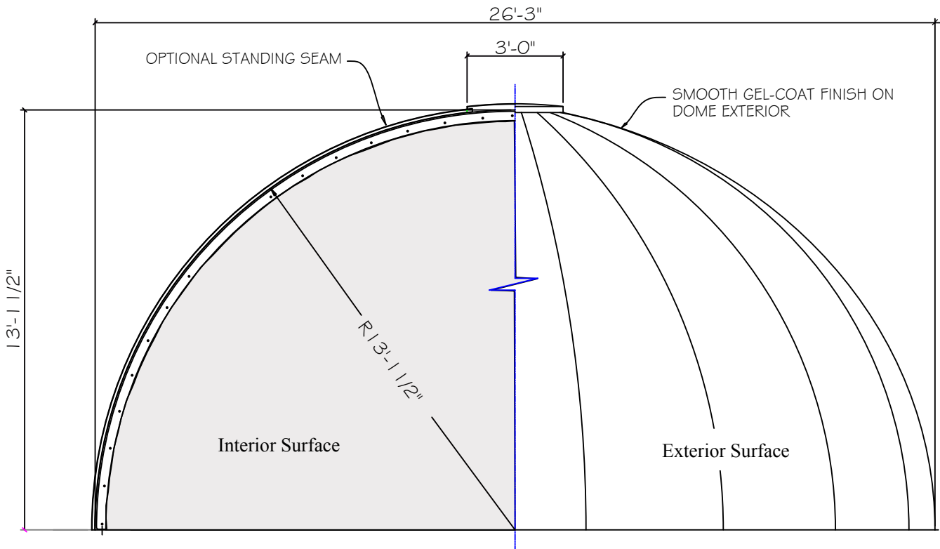
SECTION / ELEV. OF ED0-507
