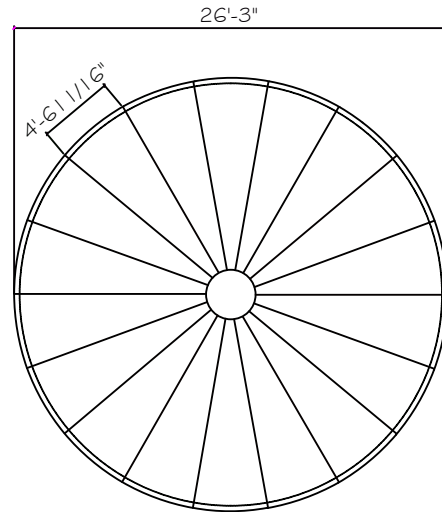
PLAN OF ED0-507
