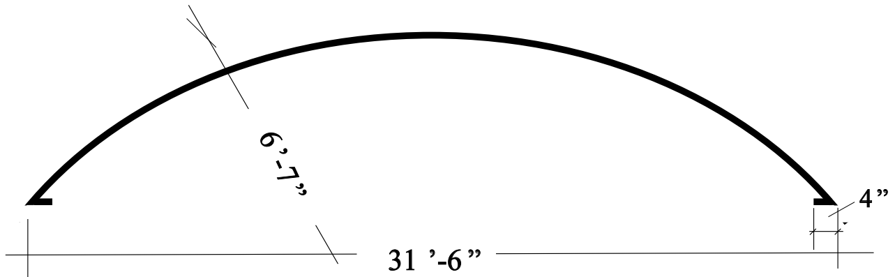
SECTION/ELEVATION OF EDO-508
