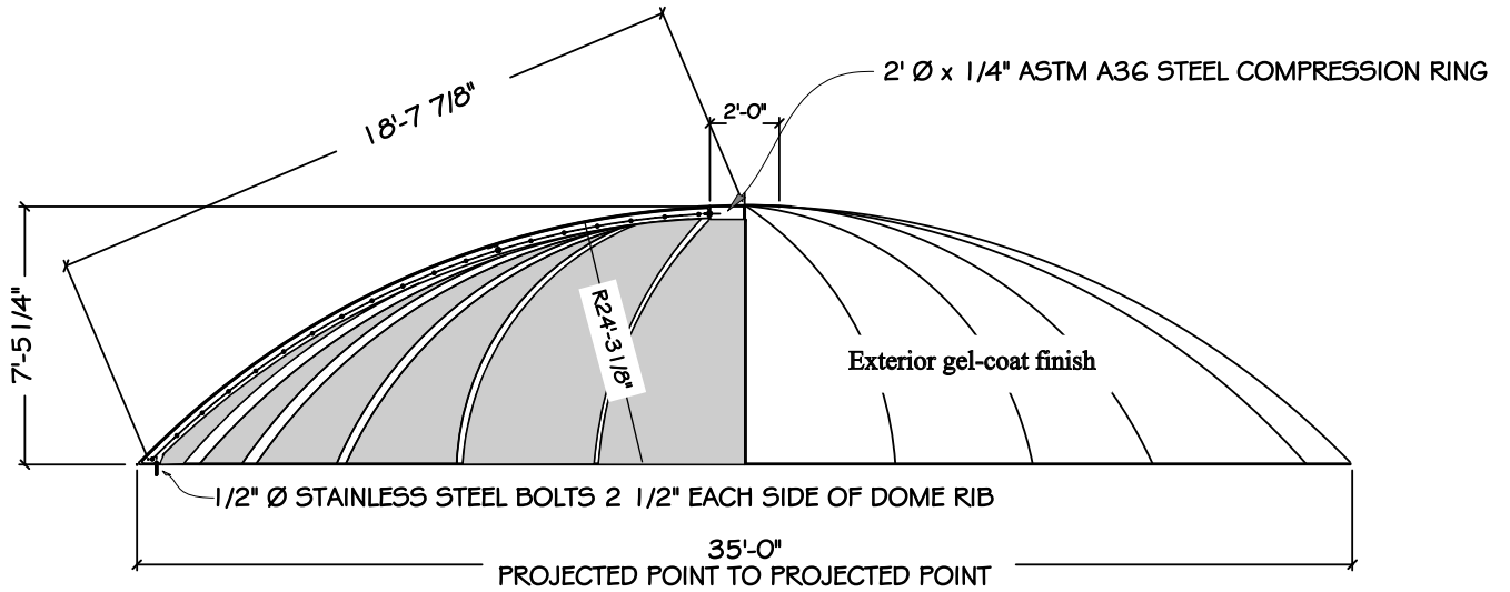
SECTION/ELEVATION OF EDO-527
