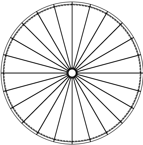
DOME PLAN VIEW
