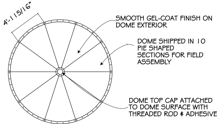
DOME PLAN DETAIL
