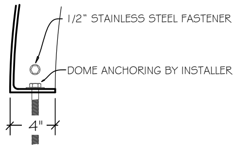
BASE BOLT FLANGE
