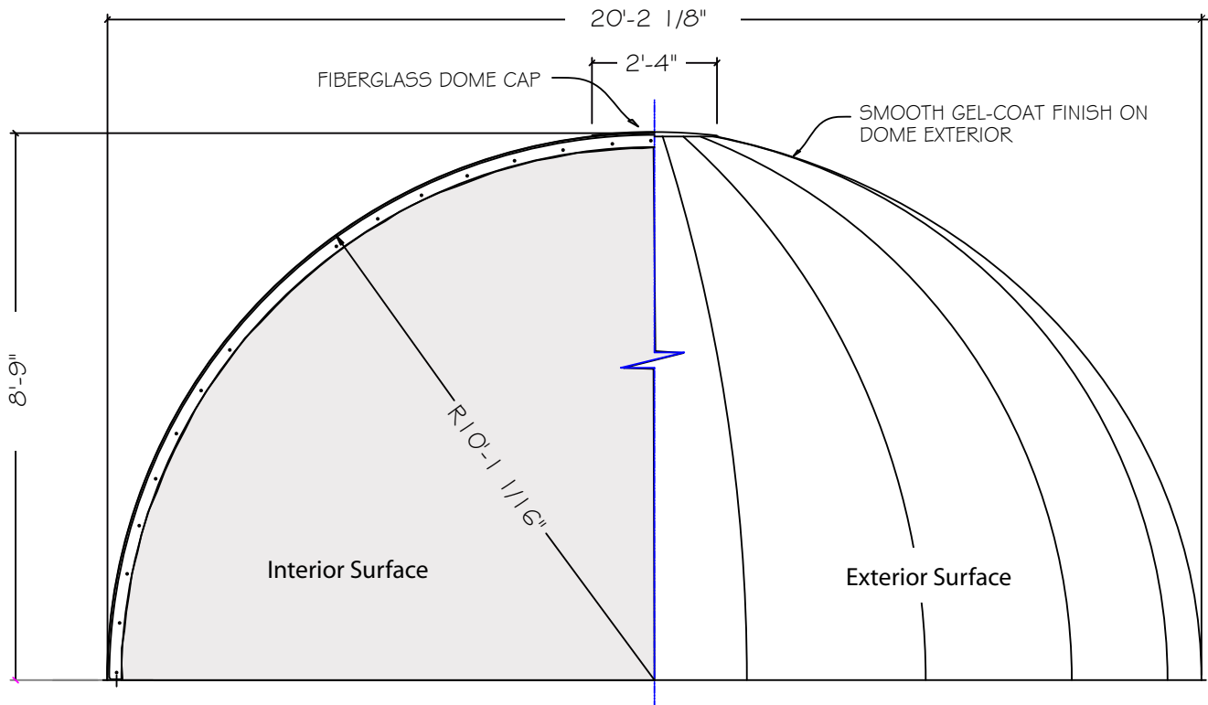
SECTION / ELEV. OF ED0-531
