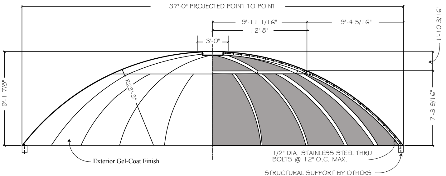
ELEVATION DETAIL
