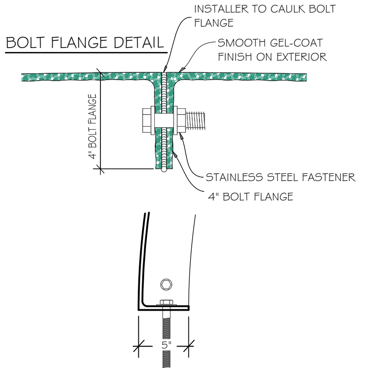
BASE BOLT FLANGE DETAIL
