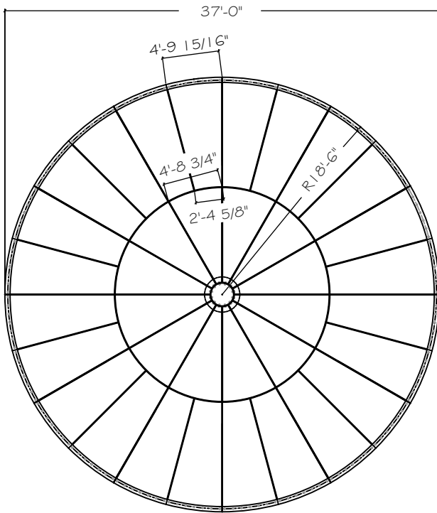
PLAN DETAIL
