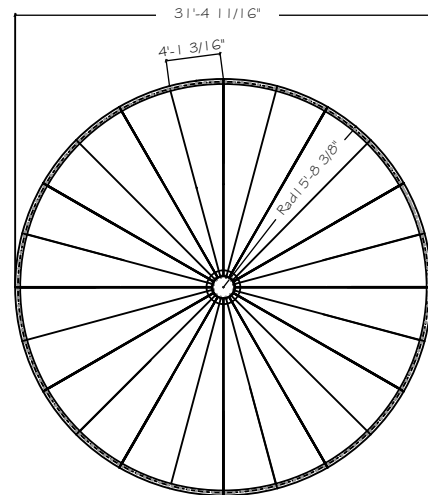
PLAN OF ED0-534 DOME
