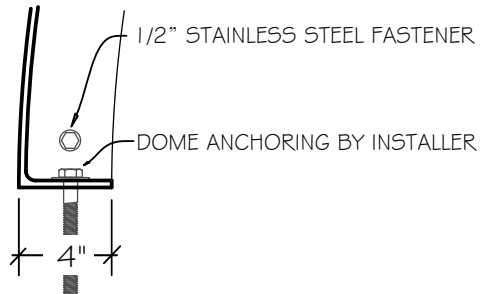
BASE BOLT FLANGE DETAIL
