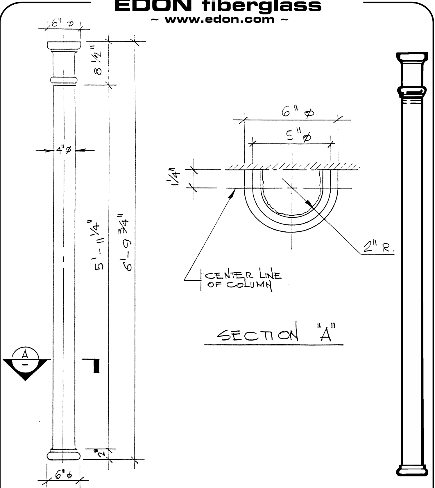
EP-101 4" DIA. TUSCAN PILASTER
