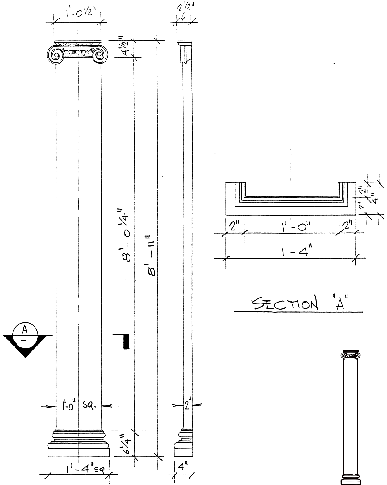
EP-102 12" SQ. ROMAN IONIC PILASTER
