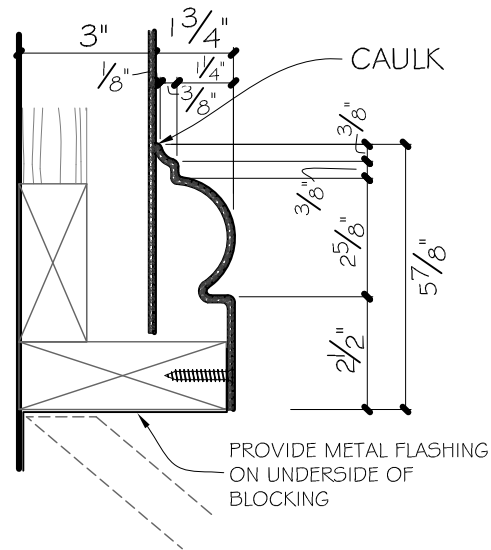
SECTION @ PILASTER BASE
