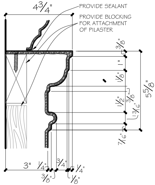
SECTION THRU CAPITAL
