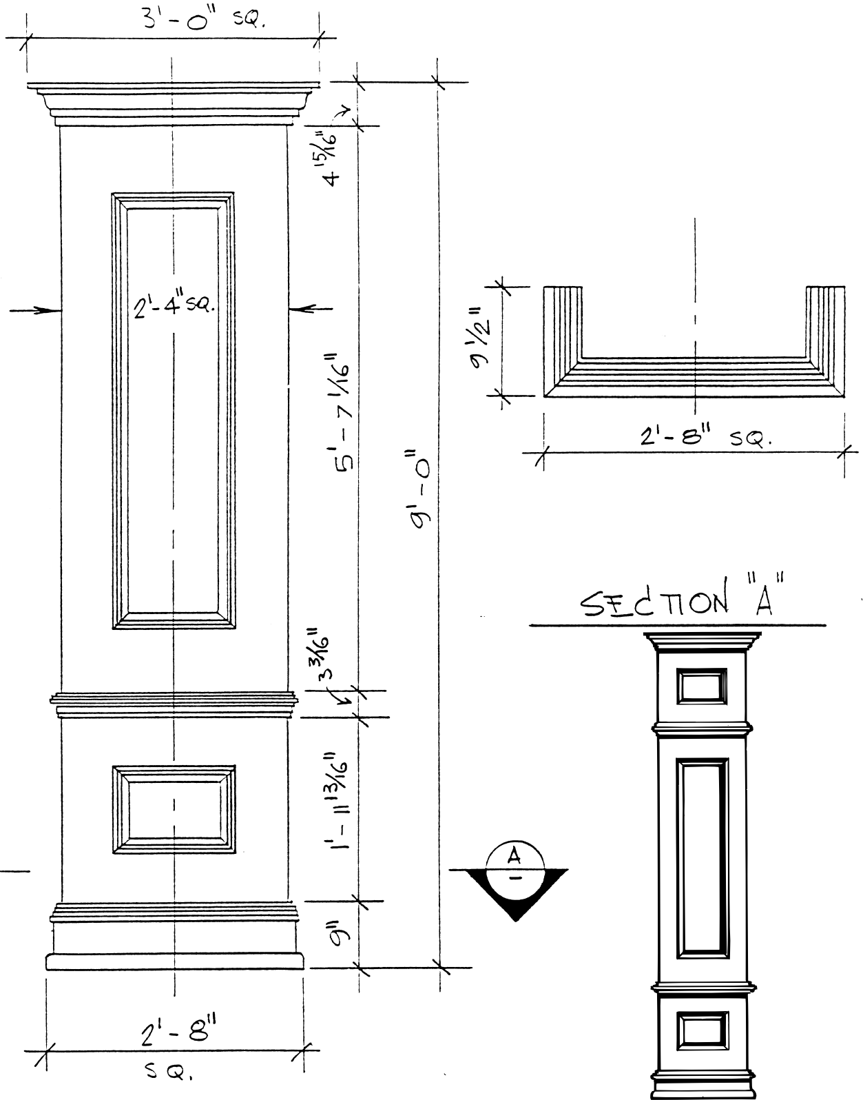
EP-110 28" SQ. ORNAMENTAL PILASTER
