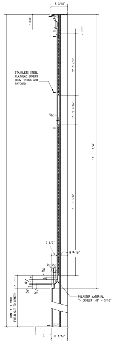
2 6 PILASTER SECTION
