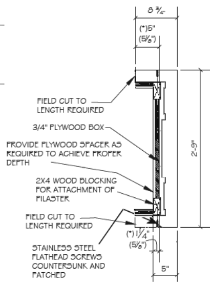
3 6 PILASTER PLAN
