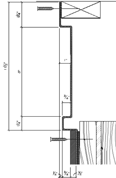
2 CAPITAL DETAILS
