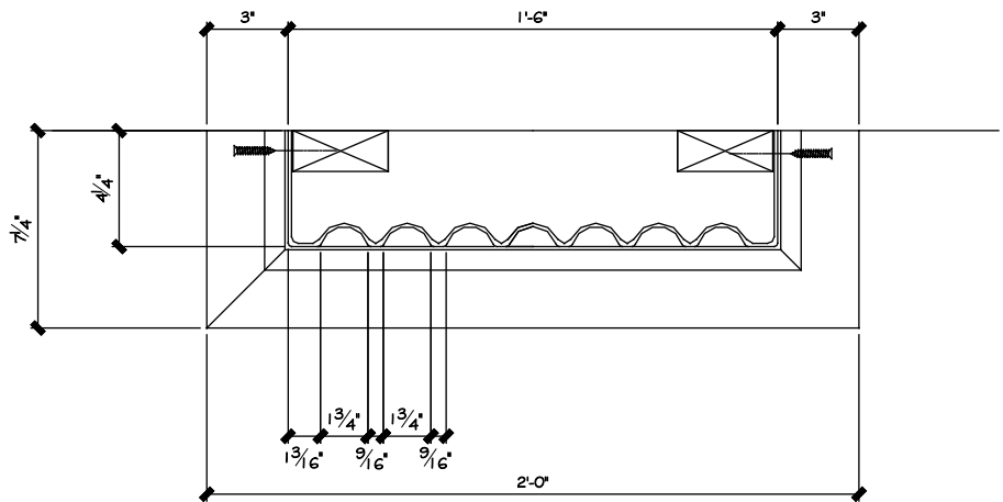
PILASTER BASE
