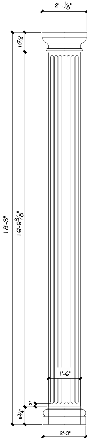
ELEV. OF EP-138 PILASTER
