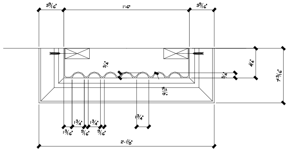
REFLECTED PLAN OF CAPITAL
