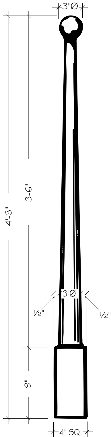
ELEVATION OF SPIRE
