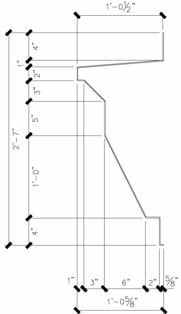
CR-529 Ornamental Cornice
