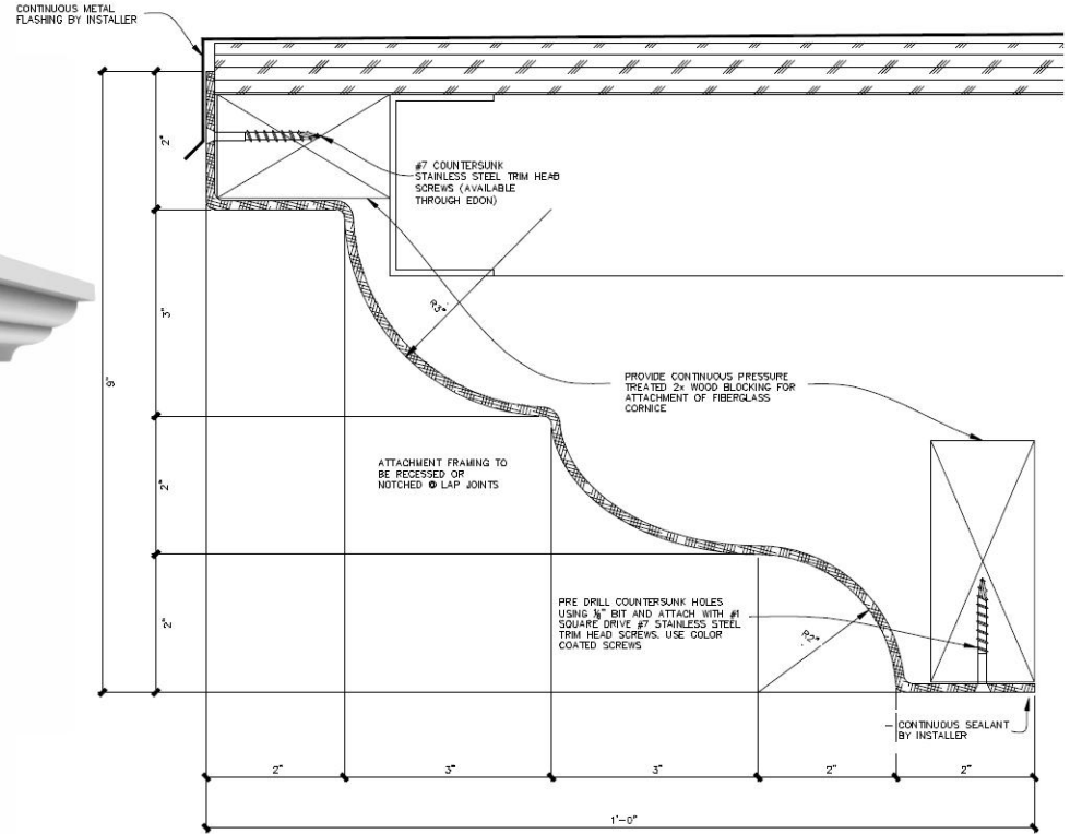
CR-552 Ornamental Cornice
