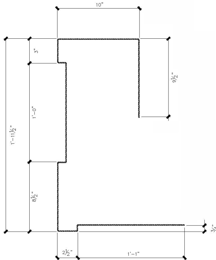
CR-553 Ornamental Cornice
