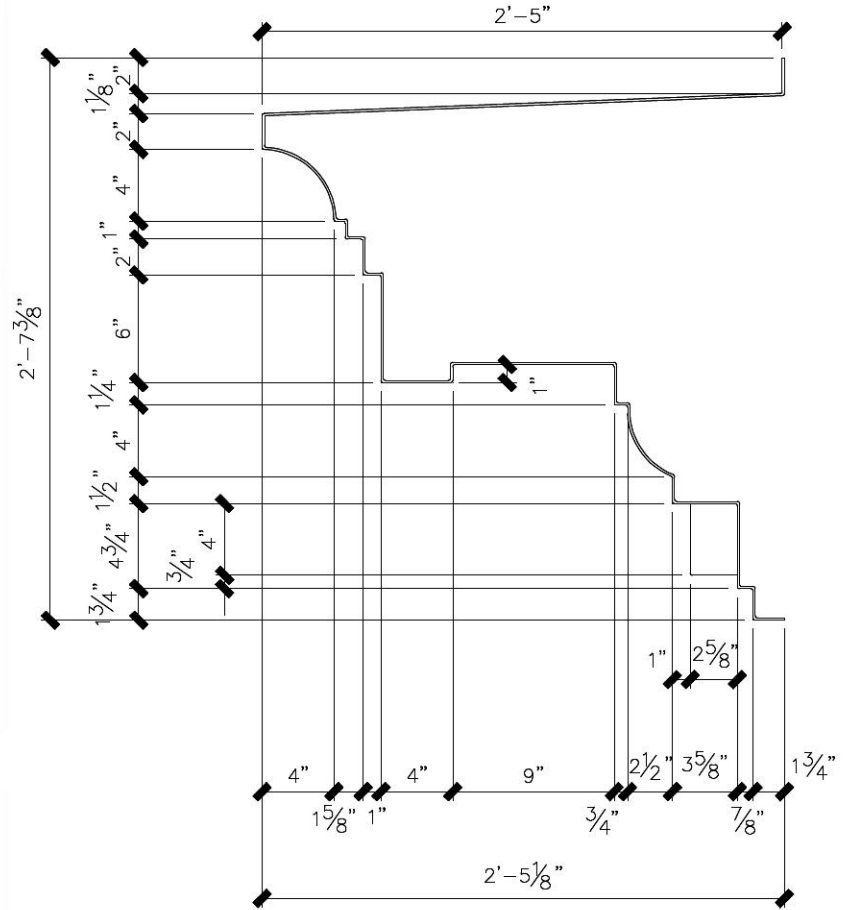
CR-591 Ornamental Cornice
